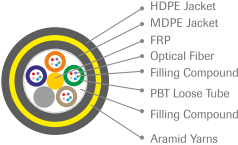
CONSTRUCTION DETAILS OF ADSS CABLE
