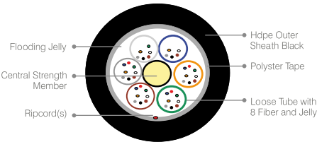
CONSTRUCTION DETAILS OF 48 FIBER
