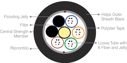
CONSTRUCTION DETAILS OF 24 FIBER
